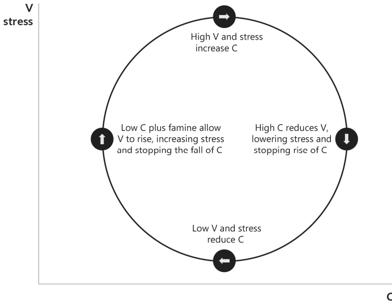
Fig. 12.5. Civilization cycle complete model.
